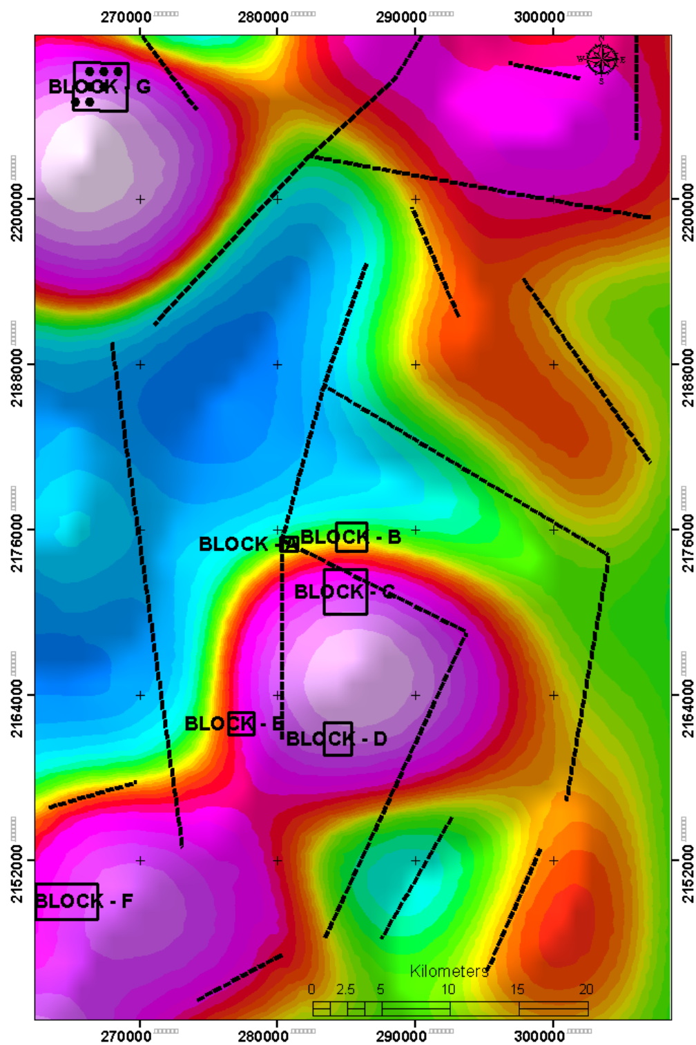
Fig. 4.1. Basement structure features in the project area, overlain upon the Horizontal Gradient
