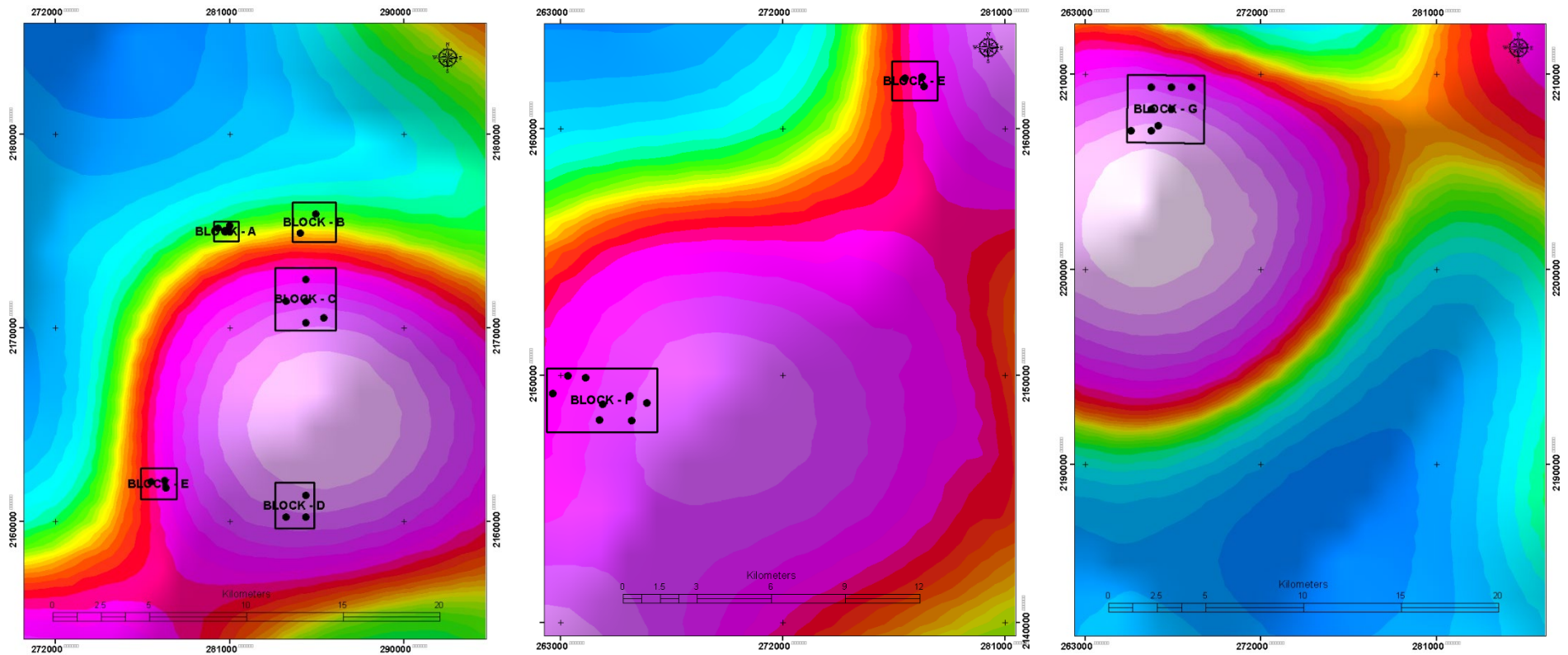
Fig. 6b. The exploration targets overlain upon the Residual Gravity Anomaly
