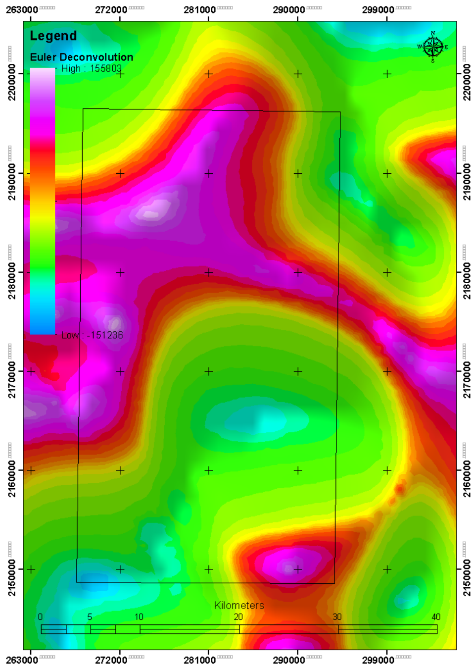
Fig. 3.6. Euler Deconvolution Depth map of the project area
