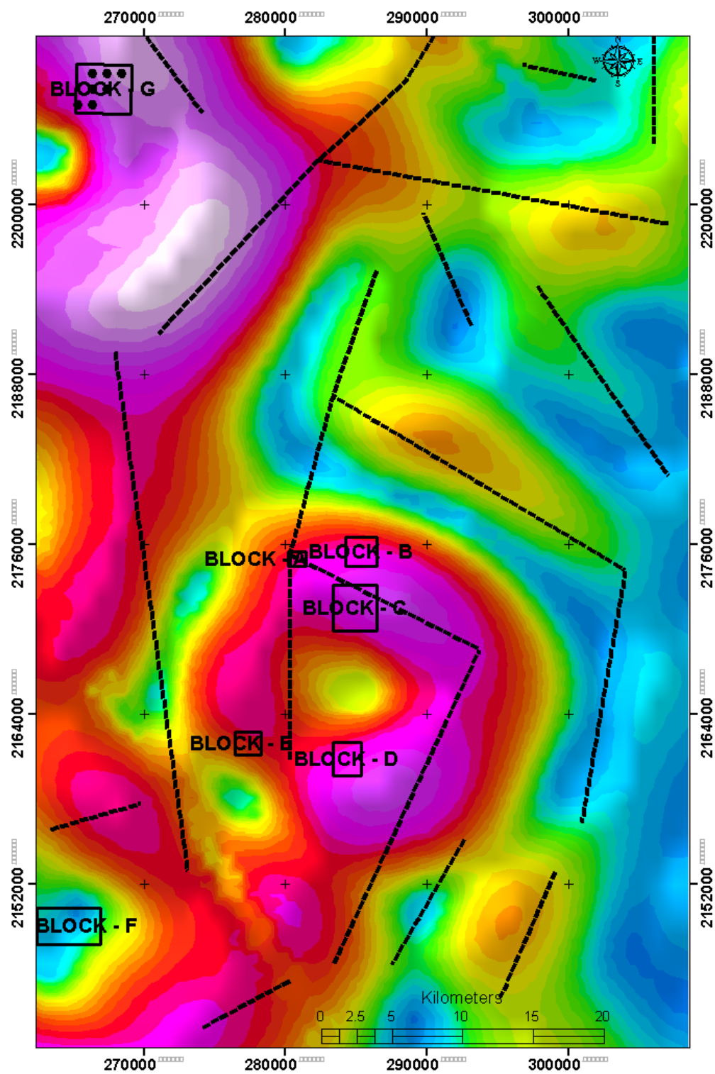
Fig. 4.2. Basement structure features in the project area, overlain upon the Residual Gravity
