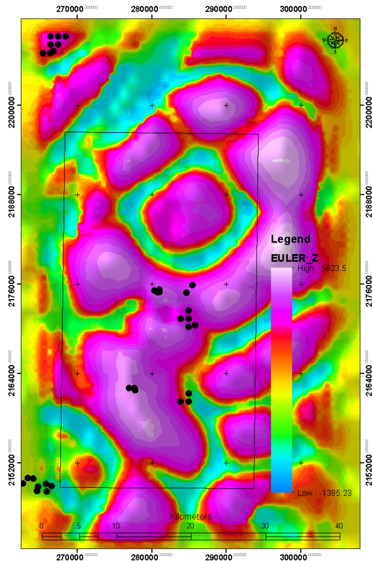
Fig. 3.5. Euler Depth map of the project area superimpose the target points
