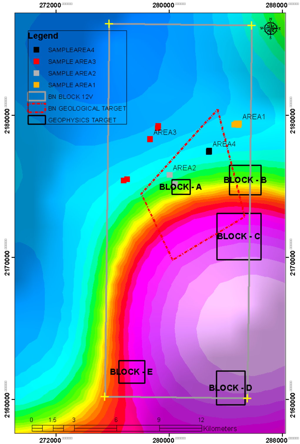
Fig. 6a. The exploration targets overlain upon the Residual Gravity Anomaly, illustrate BN Block 12V, BN polygon target area and location of geochemical samples
