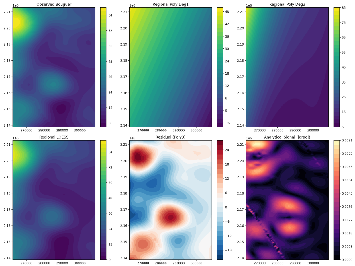
Fig. 5.1. Satellite Gravity Data model
